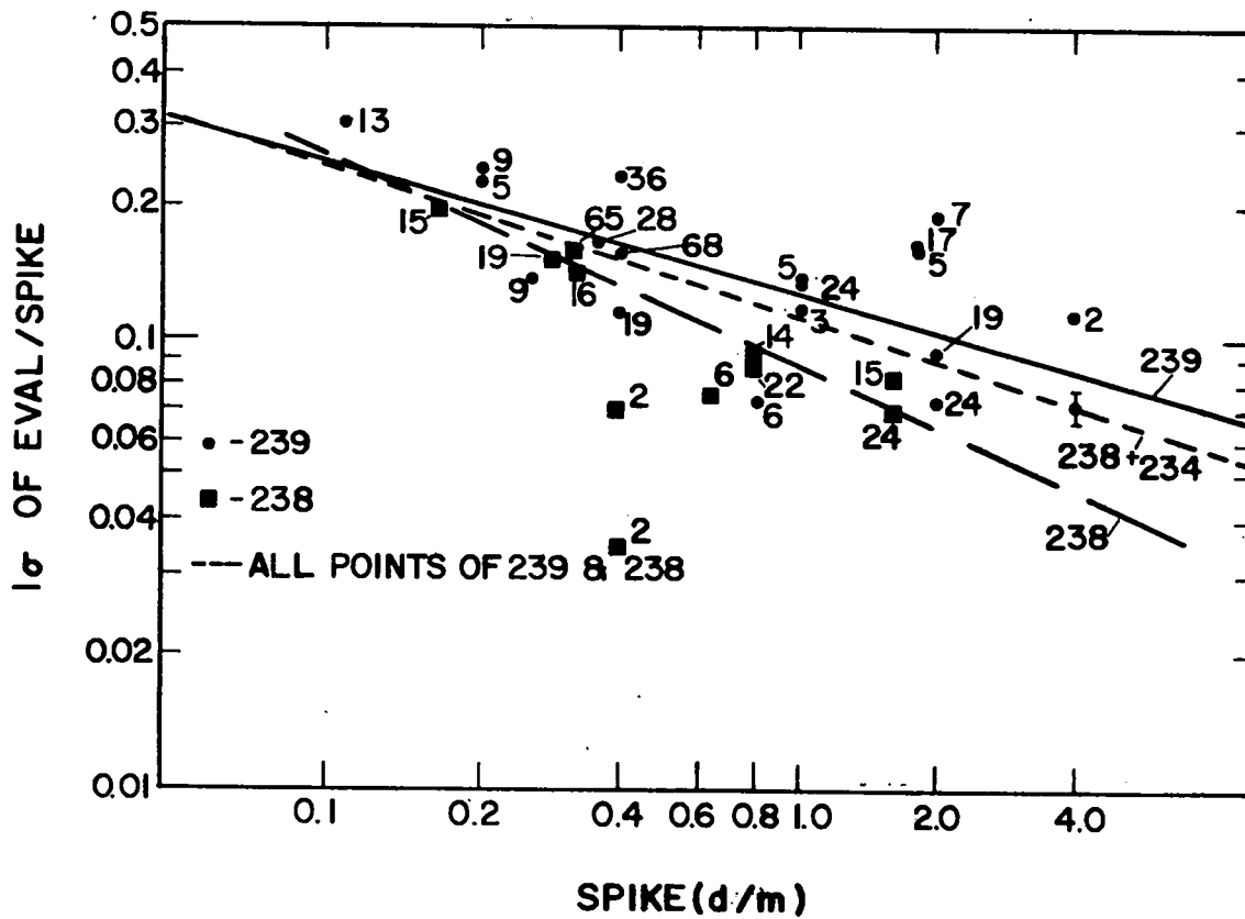
Fig. C-2. Single- \sigma values vs overspike.
